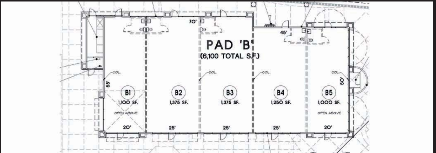
PRELIMINARY ELEVATION AND LEASING PLAN: PAD 'B', FLOOR PLAN, 6,100 S.F.
