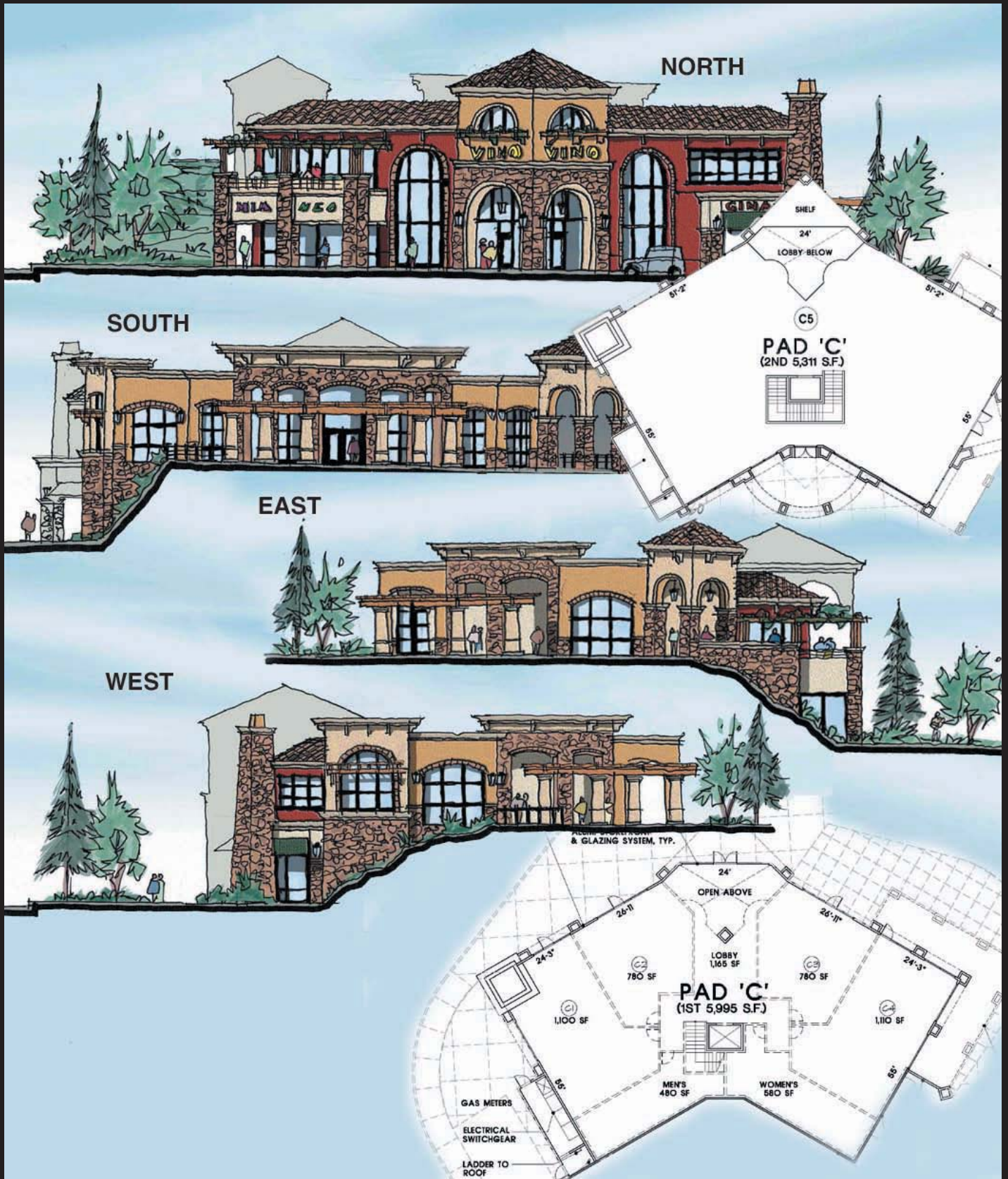
PRELIMINARY ELEVATION AND LEASING PLAN: PAD 'C', FLOOR PLAN, LV 1 - 5,995 S.F., LV 2 - 5,311 S.F.
